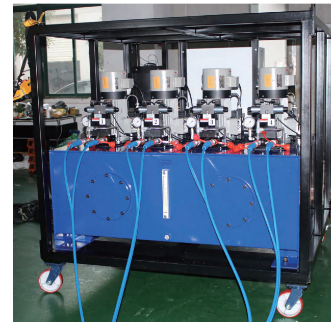
Four Point Synchronous Lifting System (Hydraulic Pump Station) 1600tons Four Point Synchronous Lifting System(1.8m stroke)
